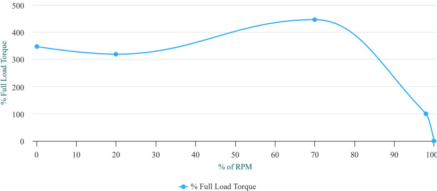
Torque Speed (T-n) Curve
